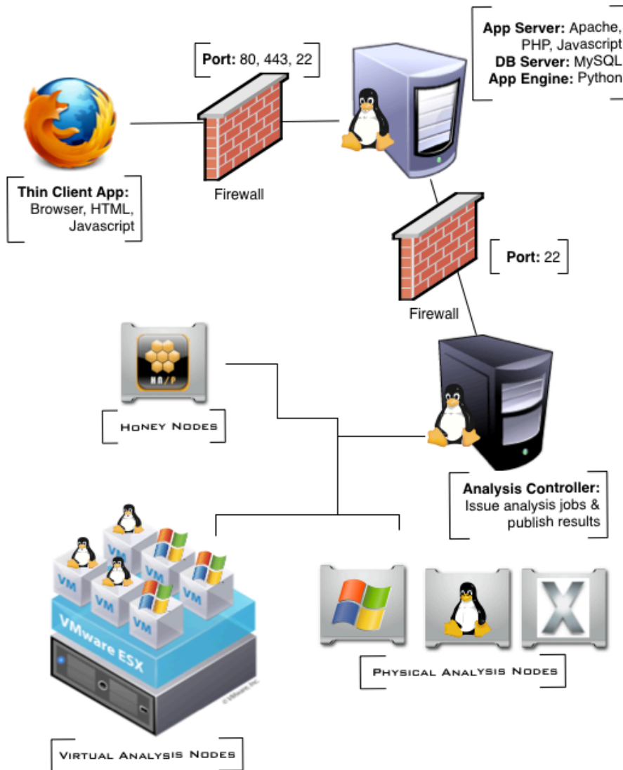
Figure 4.5.1: MyZoo Conceptual Design
